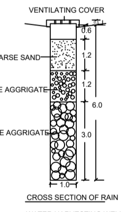
CROSS SECTION OF RAIN WATER HARVESTING WELL
